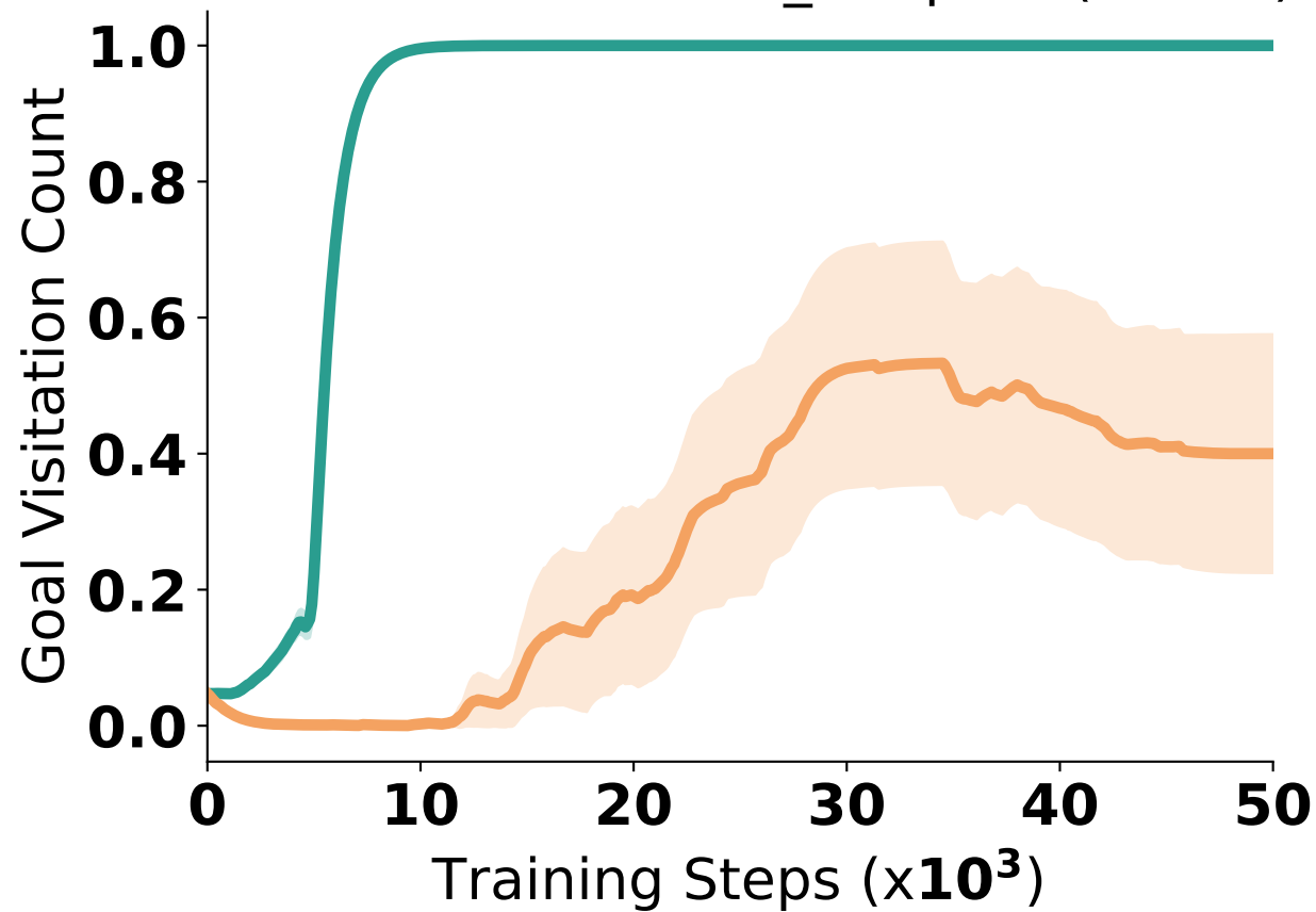
Gridworld-Bottleneck_NExperts(80.0%)
